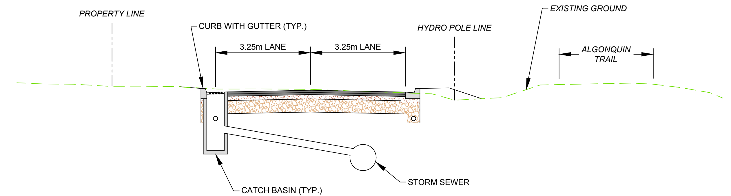
ROAD WITH CURB ON BOTH SIDES STATION 11+100 TO 12+580
