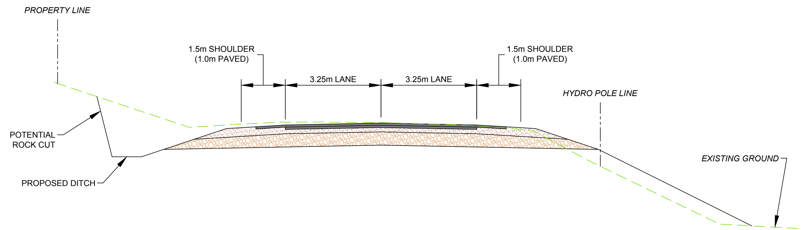
ROAD WITH SHOULDER ON BOTH SIDES STATION 10+425 (TONER RD) TO 10+950
