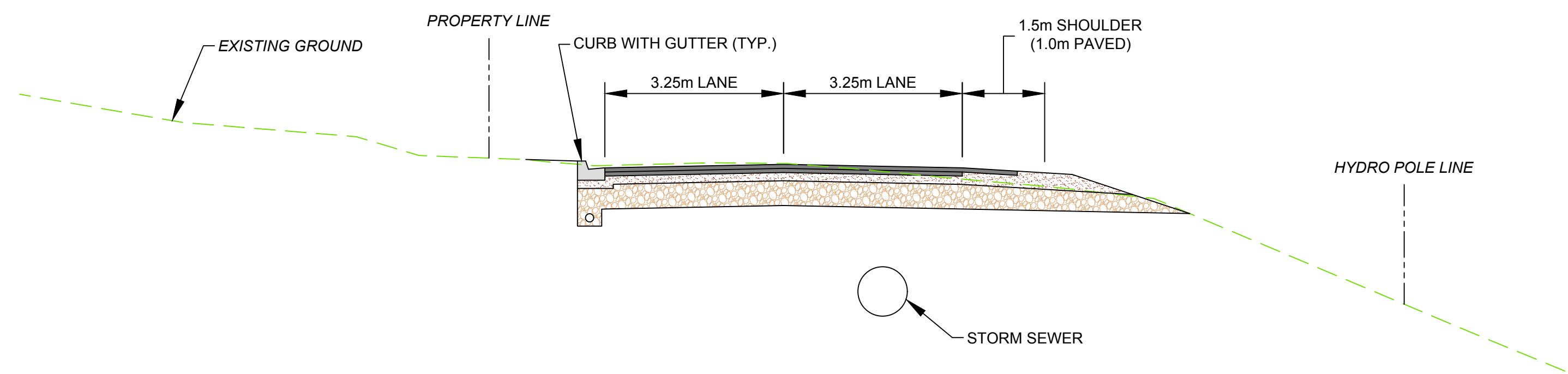
ROAD WITH CURB ON ONE SIDE STATION 10+950 TO 11+100
